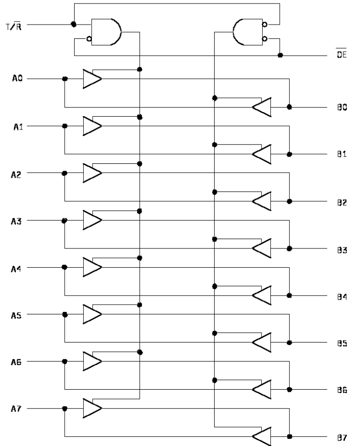
FIGURE 3. Logic diagram.
