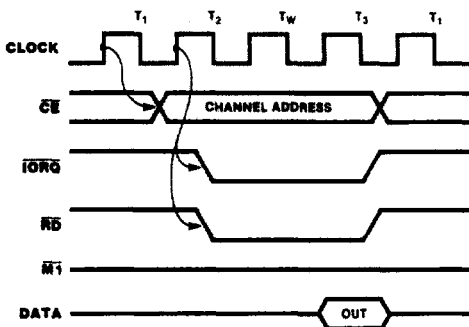
Figure 5. Read Cycle
