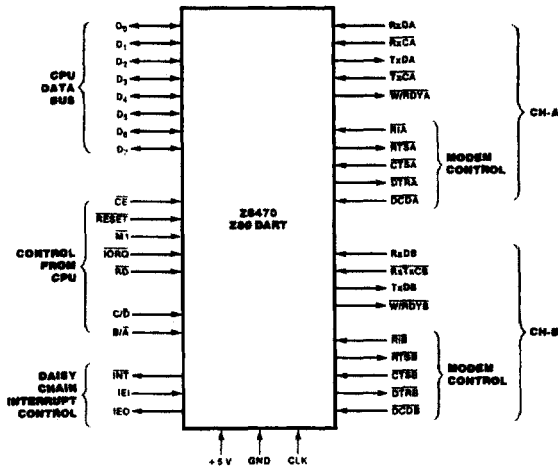
Figure 1. Pin Functions
