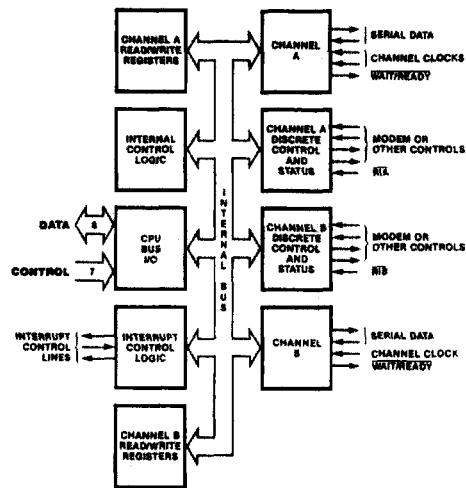
Figure 3. Block Diagram
