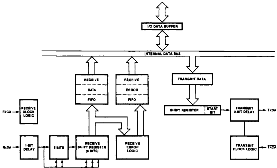
Figure 4. Data Path
