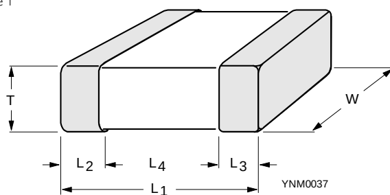
Fig. 2 Surface mounted multilayer ceramic capacitor dimension
