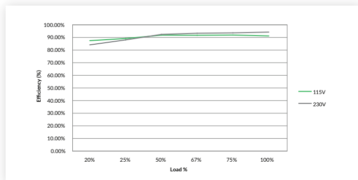
Figure 5 GCS250PS48
