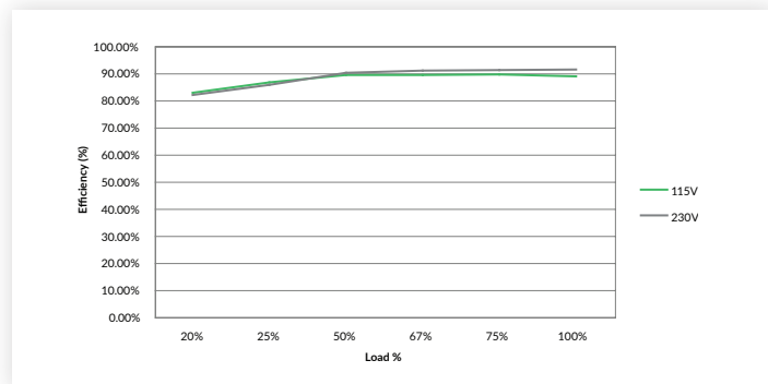
Figure 3 GCS250PS12
