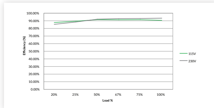
Figure 4 GCS250PS24
