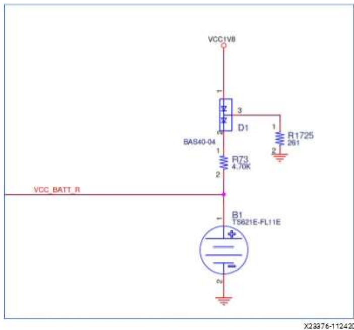
Figure: Encryption Key Backup Circuit
