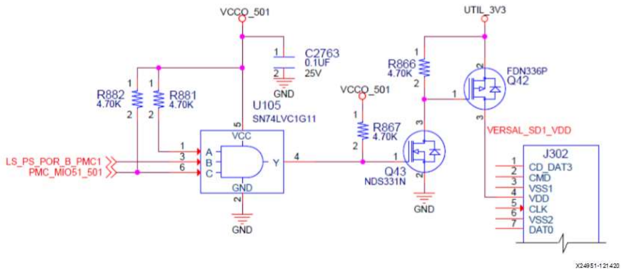
Figure: SD Socket J302 Power Control
