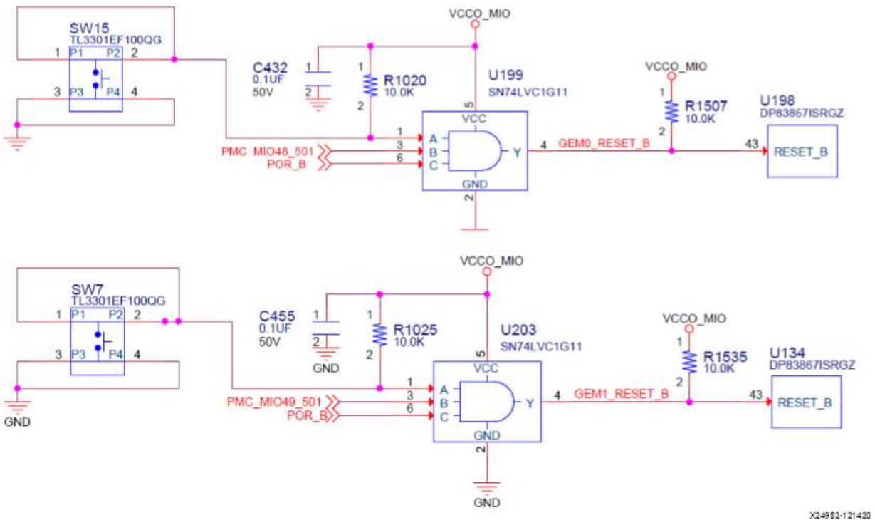
Figure: Ethernet PHY Reset Circuit
