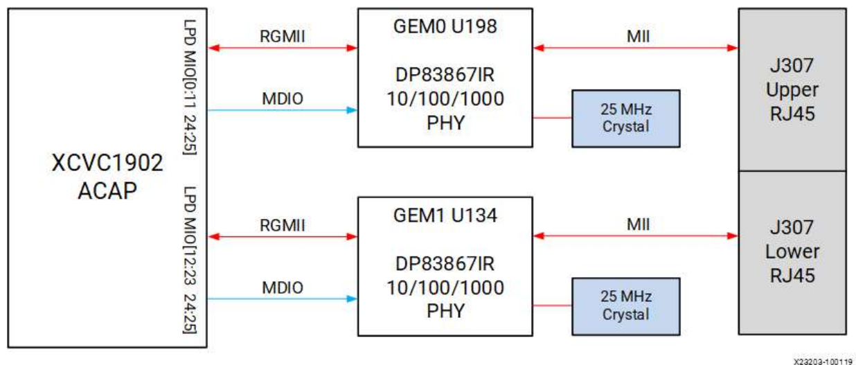
Figure: Dual RGMII Ethernet
