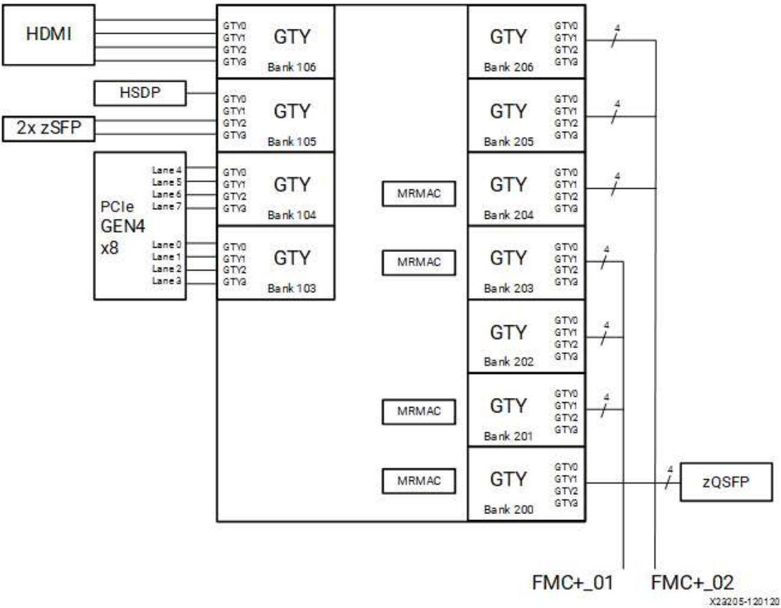
Figure: VCK190 GTY Connections
