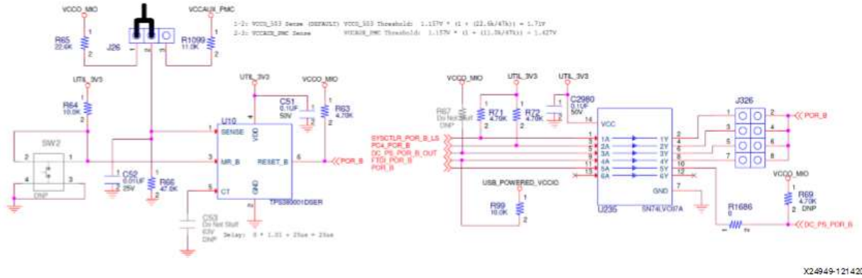
Figure: POR_B Reset Circuit
