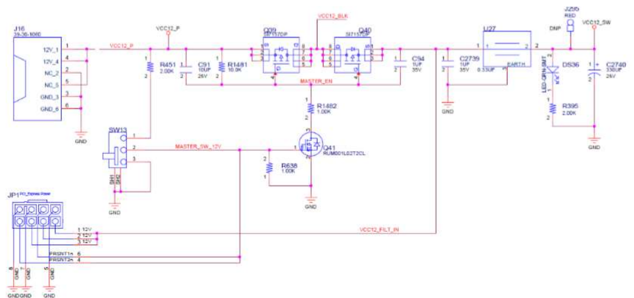
Figure: Power Input
