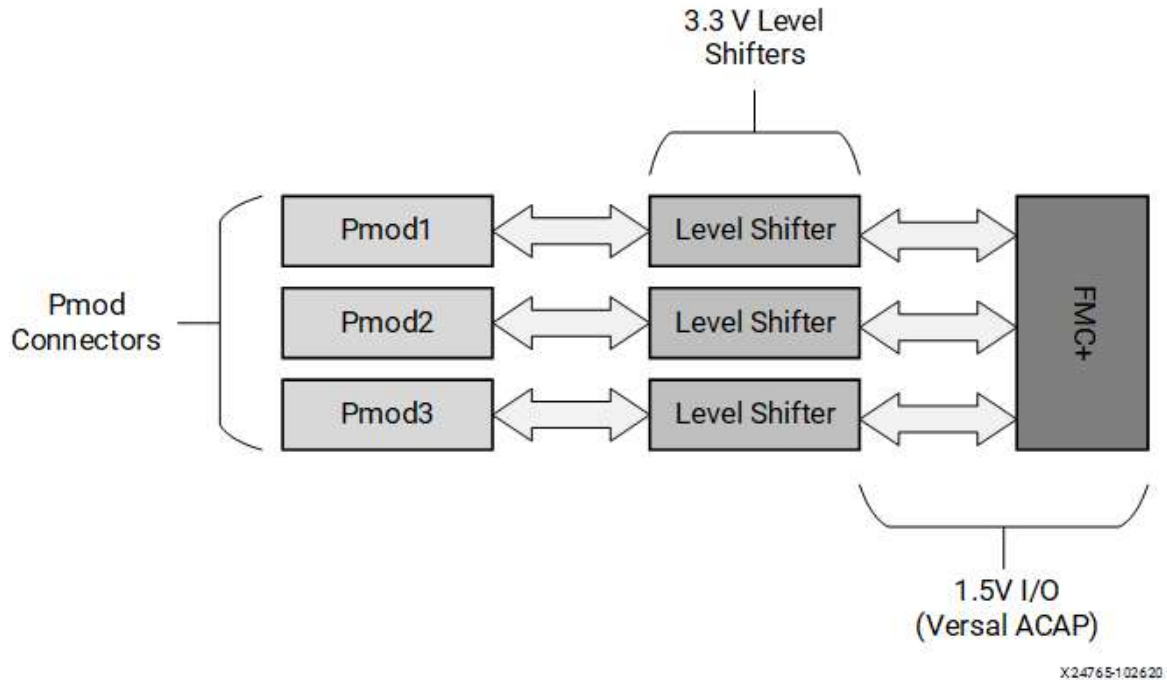
Figure: Pmod FMC Block Diagram
