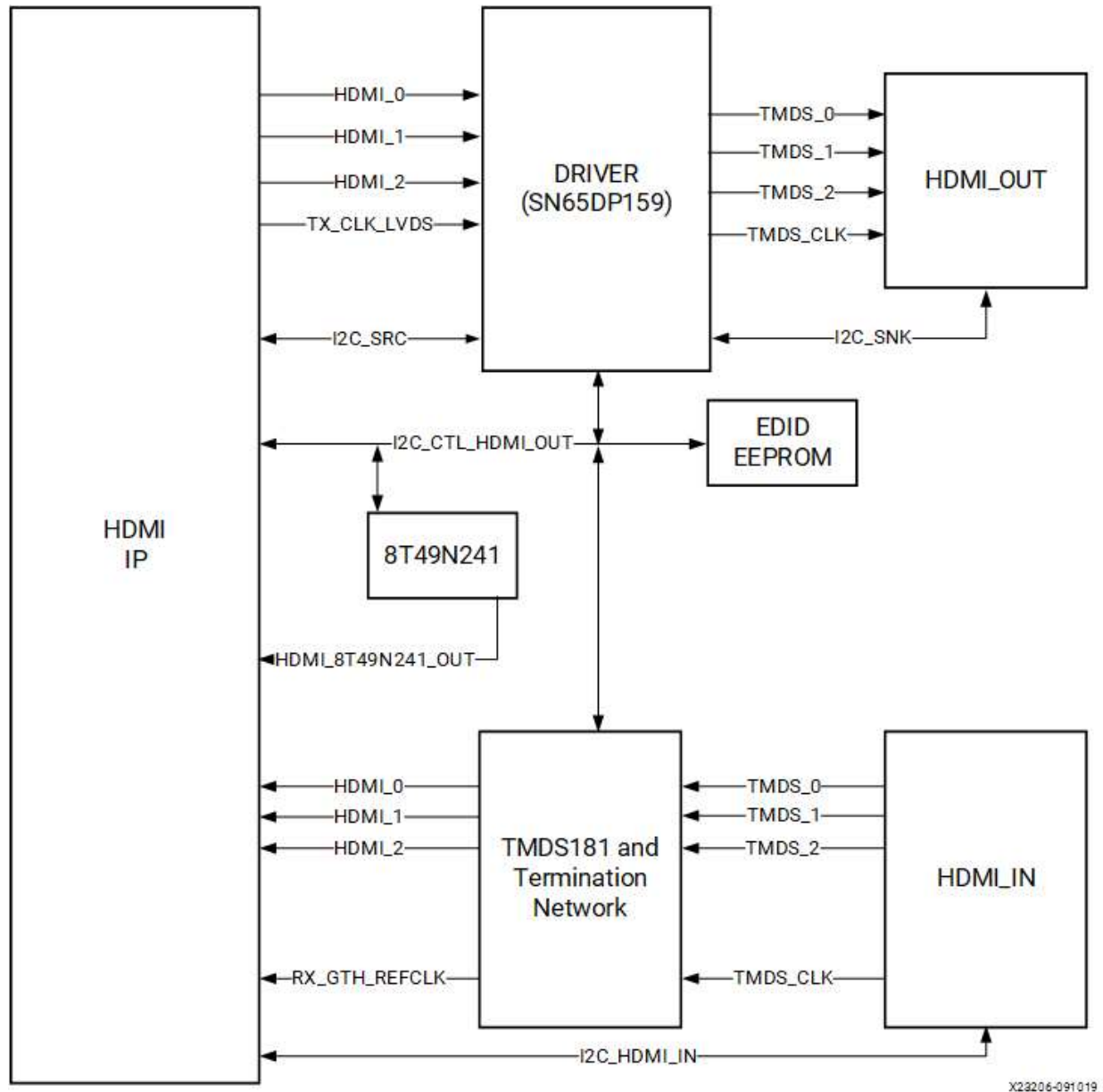
Figure: HDMI Interface Block Diagram
