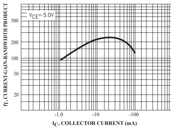
Figure 12. Current-Gain-Bandwidth Product
