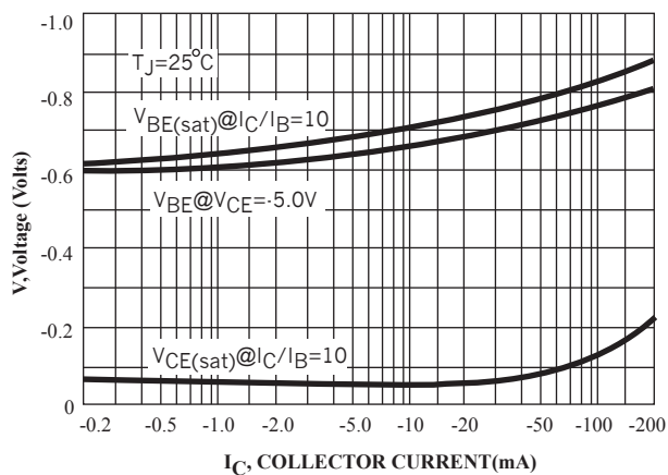
Figure 8. "ON" Voltage
