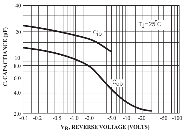
Figure 11. Capacitance
