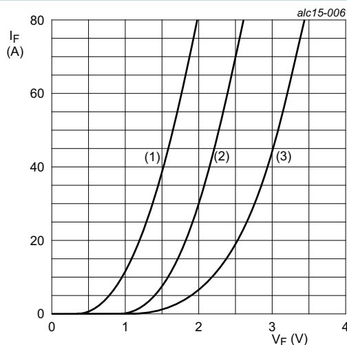
V_o = 1.620\text{ V}; R_s = 0.0132\text{ }\Omega (1) T_j = 150\text{ }^\circ\text{C}; typical values (2) T_j = 150\text{ }^\circ\text{C}; maximum values (3) T_j = 25\text{ }^\circ\text{C}; maximum values
