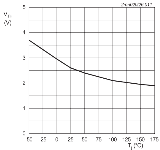
V_{DS} = 10\text{ V} ; I_{DS} = 20\text{ mA} Fig. 11. Threshold voltage as a function of junction temperature
