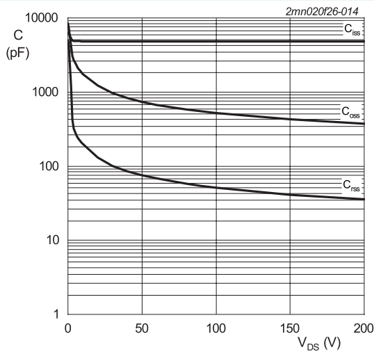
V_{DS} = 0 - 200 \text{ V} T_j = 25 \text{ }^\circ\text{C}; V_{AC} = 100 \text{ mV}; f = 1 \text{ MHz} Fig. 14. Input, output and reverse transfer capacitances as a function of drain-source voltage; typical values
