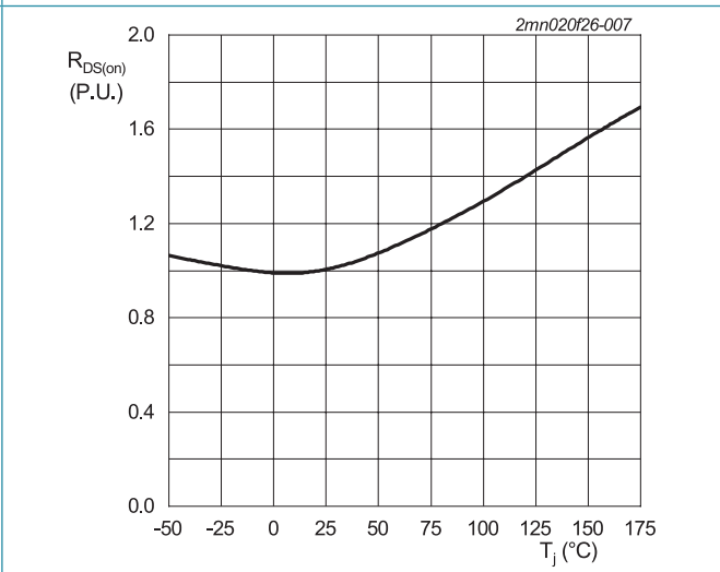
I_{DS} = 50\text{ A}; V_{GS} = 18\text{ V}; t_p < 200\ \mu\text{s} Fig. 7. Normalized drain-source on-state resistance as a function of junction temperature
