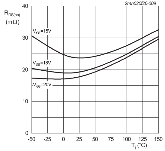
I_{DS} = 50\text{ A} ; t_p < 200\ \mu\text{s} Fig. 9. Drain-source on-state resistance as a function of junction temperature
