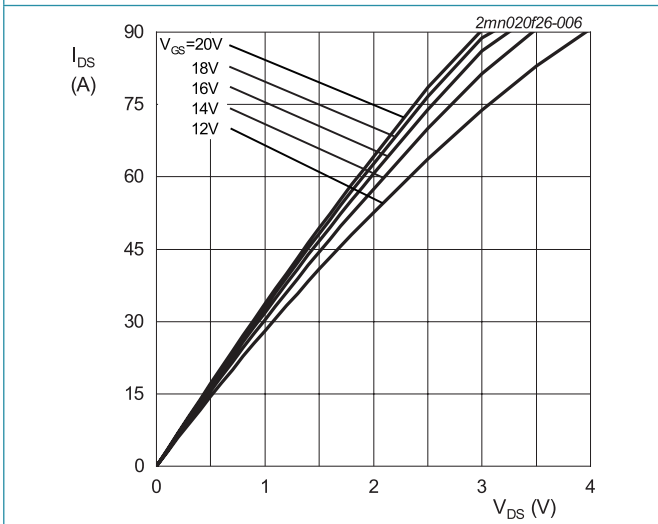
T_j = 175\text{ °C}; t_p < 200\ \mu\text{s} Fig. 6. Output characteristics; drain current as a function of drain-source voltage; typical values
