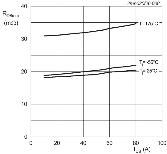
V_{GS} = 18\text{ V} ; t_p < 200\ \mu\text{s} Fig. 8. Drain-source on-state resistance as a function of drain current; typical values
