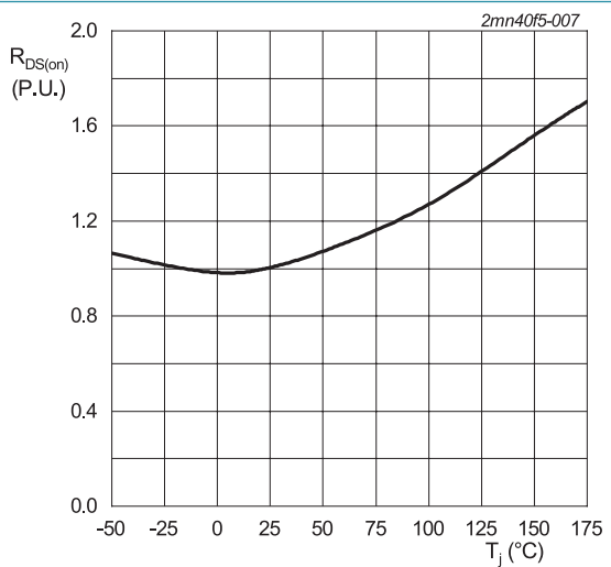
I_{DS} = 35\text{ A}; V_{GS} = 18\text{ V}; t_p < 200\ \mu\text{s} Fig. 7. Normalized drain-source on-state resistance as a function of junction temperature
