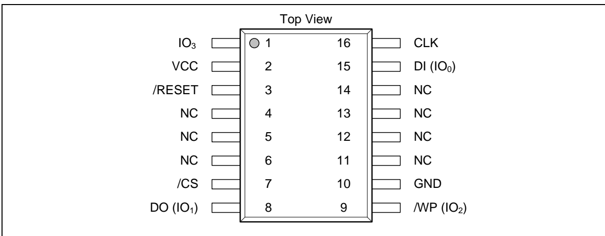
Figure 1c. W25Q64JV Pin Assignments, 16-pin SOIC 300-mil (Package Code SF)
