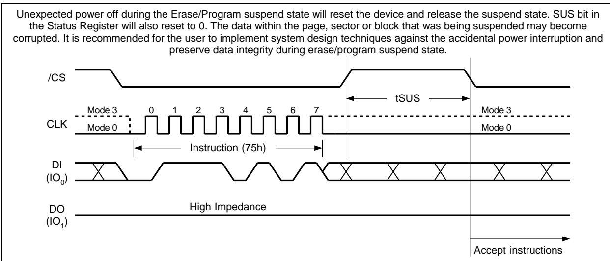
Figure 35. Erase/Program Suspend Instruction
