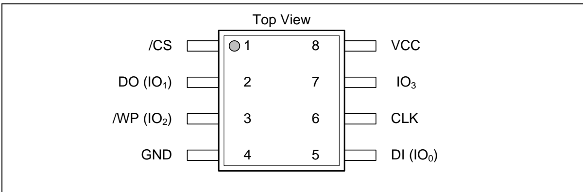
Figure 1a. W25Q64JV Pin Assignments, 8-pin SOIC 208-mil (Package Code SS)
