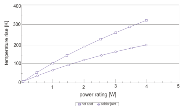
TEMPERATURE RISE
