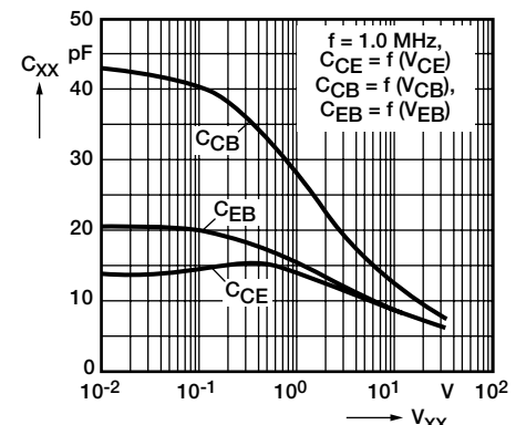
Fig. 11 - Transistor Capacitance
