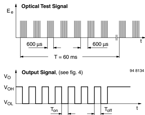
Figure 3. Output Function
