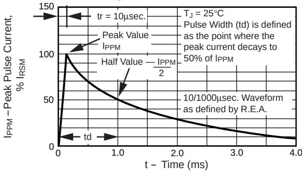
Fig. 3 – Pulse Waveform
