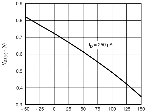
T_J - Junction Temperature (°C) Threshold Voltage
