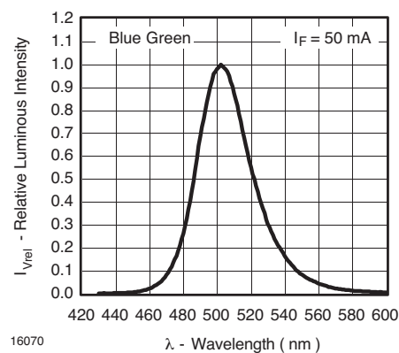
Figure 54. Relative Intensity vs. Wavelength
