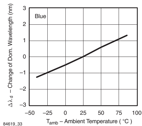
Figure 57. Change of Dominant Wavelength vs. Ambient Temperature
