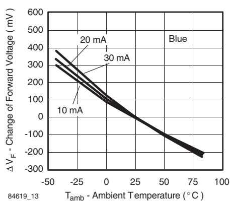
Figure 55. Change of Forward Voltage vs. Ambient Temperature
