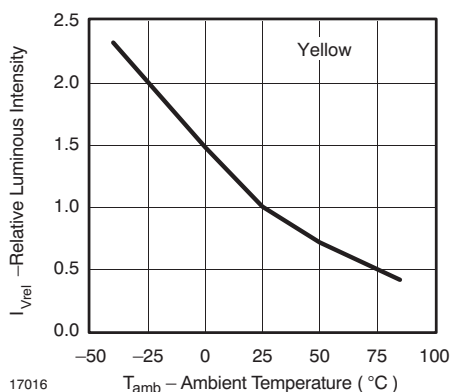
Figure 23. Relative Luminous Intensity vs. Ambient Temperature
