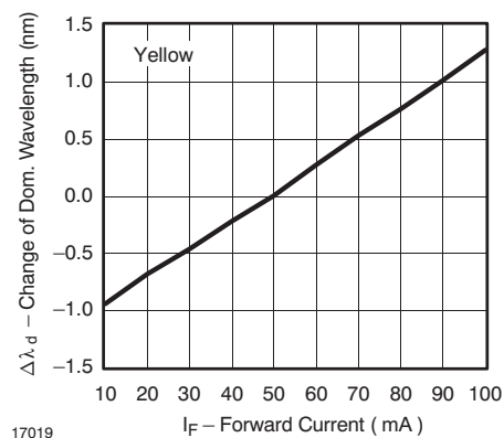
Figure 26. Change of Dominant Wavelength vs. Forward Current
