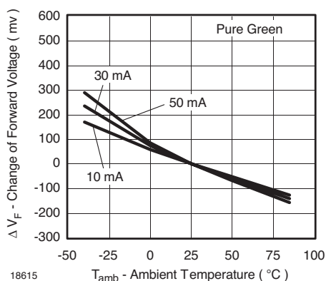
Figure 35. Change of Forward Voltage vs. Ambient Temperature
