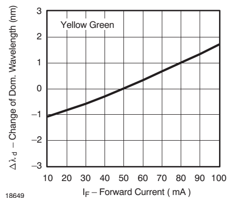
Figure 32. Change of Dominant Wavelength vs. Forward Current
