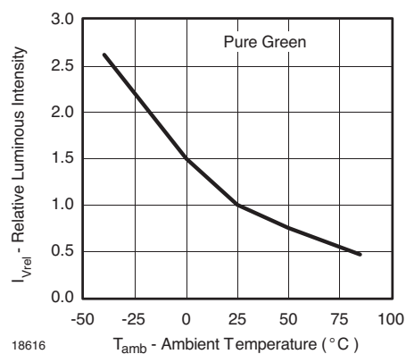
Figure 36. Relative Luminous Intensity vs. Ambient Temperature
