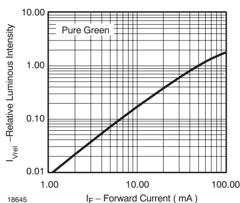
Figure 38. Relative Luminous Flux vs. Forward Current
