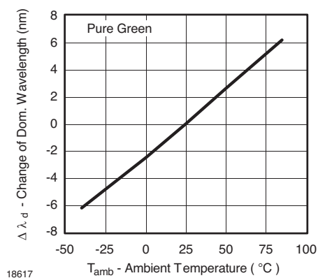
Figure 37. Change of Dominant Wavelength vs. Ambient Temperature
