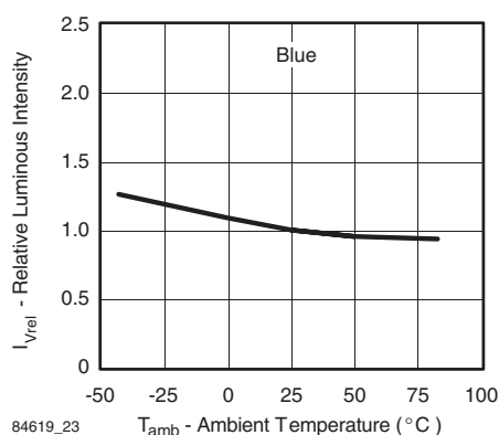
Figure 56. Relative Luminous Intensity vs. Ambient Temperature
