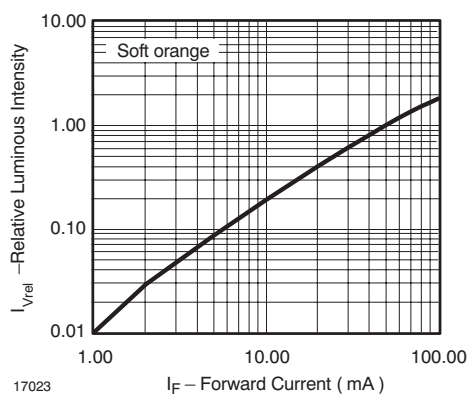
Figure 19. Relative Luminous Flux vs. Forward Current
