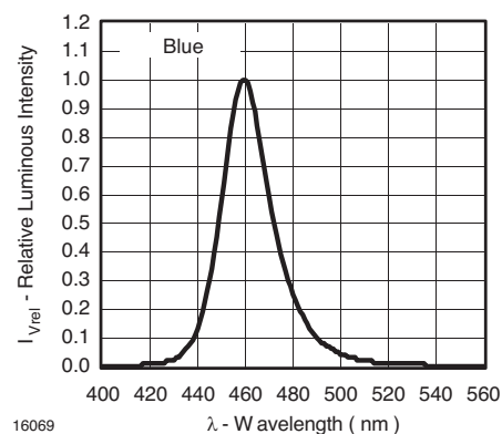
Figure 59. Relative Intensity vs. Wavelength
