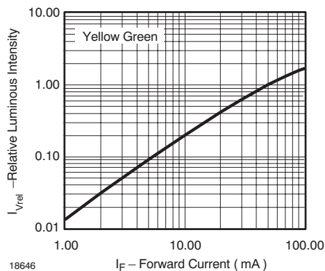
Figure 31. Relative Luminous Flux vs. Forward Current
