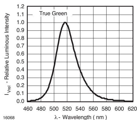
Figure 48. Relative Intensity vs. Wavelength
