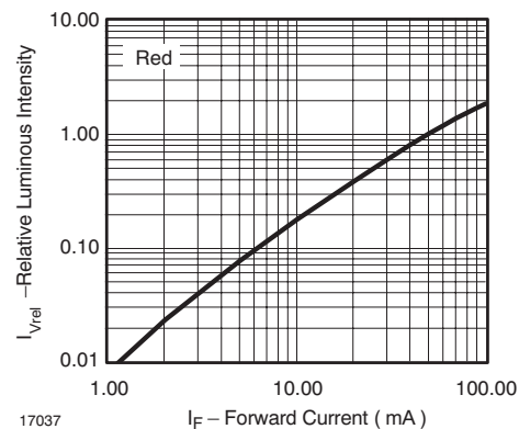
Figure 13. Relative Luminous Flux vs. Forward Current
