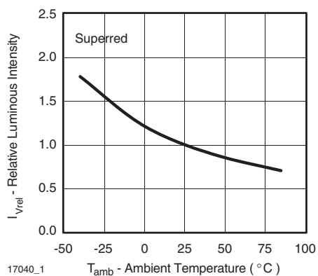
Figure 4. Relative Luminous Intensity vs. Ambient Temperature
