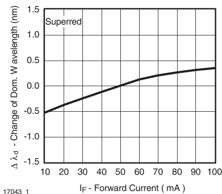
Figure 7. Change of Dominant Wavelength vs. Forward Current
