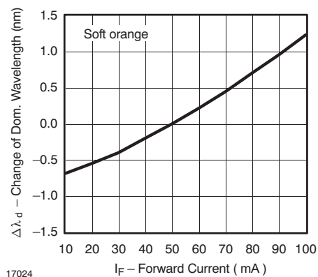
Figure 20. Change of Dominant Wavelength vs. Forward Current
