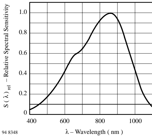
94 8348 Figure 10. Relative Spectral Sensitivity vs. Wavelength
