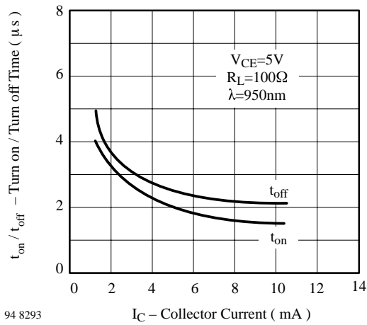
94 8293 Figure 9. Turn On/Turn Off Time vs. Collector Current
