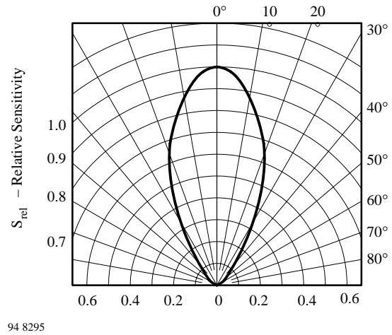
94 8295 Figure 11. Relative Radiant Sensitivity vs. Angular Displacement
