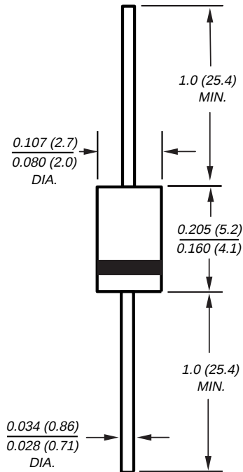
DO-204AL (DO-41 Plastic)
