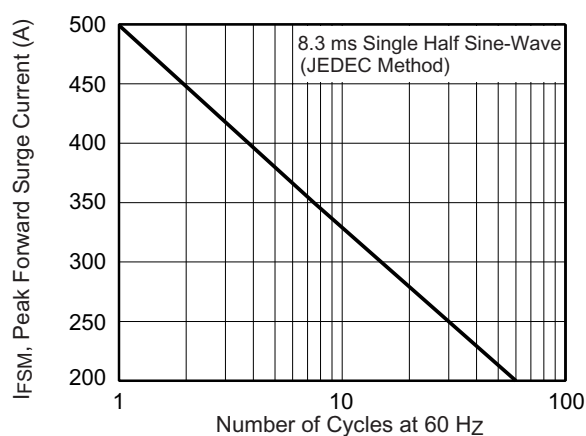
Figure 6. Maximum Non-repetitive Forward Surge Current
