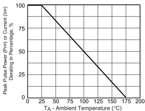
Figure 2. Pulse Power Derating Curve
