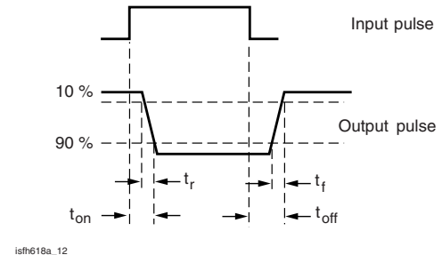
Fig. 3 - Test Circuit and Waveforms
