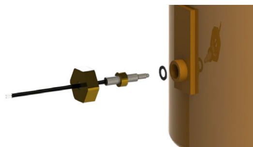
Fig. 1 - Mounting example with sealing ring and screw
