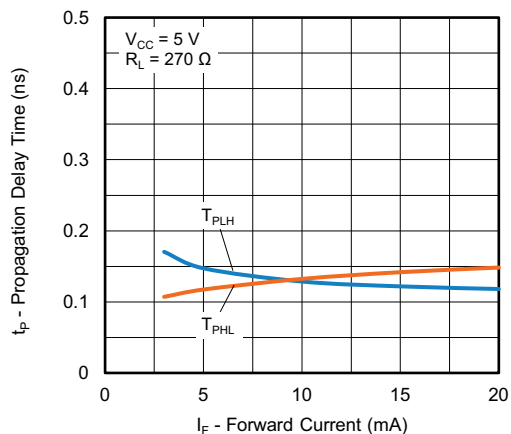
Fig. 9 - Propagation Delay Time vs. Forward Current
