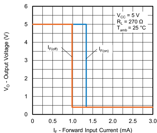
Fig. 13 - Output Voltage vs. Forward Input Current
