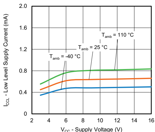
Fig. 11 - Low Level Supply Current vs. Supply Voltage
