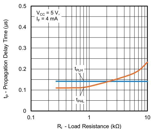
Fig. 10 - Propagation Delay Time vs. Load Resistance
