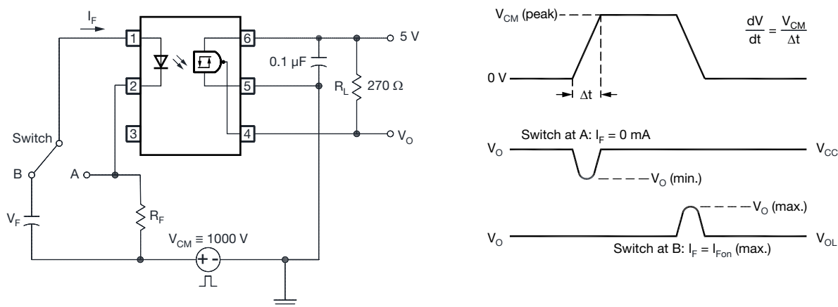
Fig. 4 - Test Circuit for Common Mode Transient Immunity
