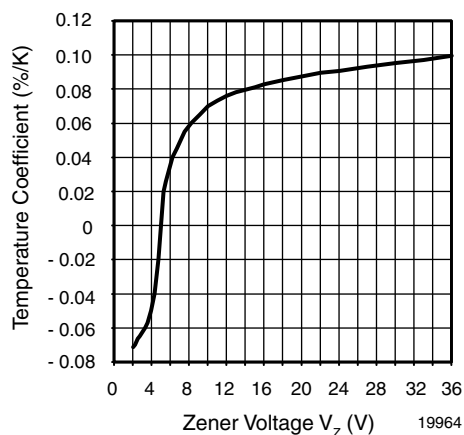
Fig. 1 - Zener Voltage Temperature Coefficient vs. Zener Voltage
