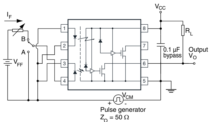
Fig. 2 - Test Circuit for Common Mode Transient Immunity
