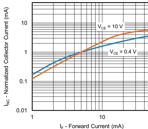
Fig. 4 - Normalized Collector Current vs. Forward Current
