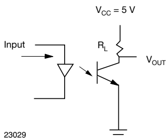
Fig. 1 - Test Circuit for Switching Characteristics
