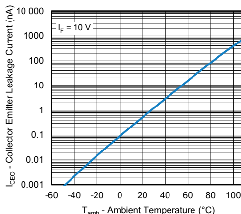
Fig. 10 - Collector Emitter Leakage Current vs. Ambient Temperature
