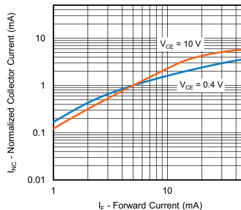
Fig. 5 - Normalized Collector Current vs. Forward Current
