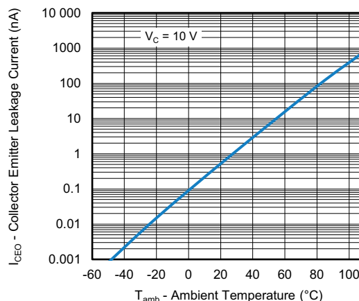
Fig. 11 - Collector Emitter Leakage Current vs. Ambient Temperature
