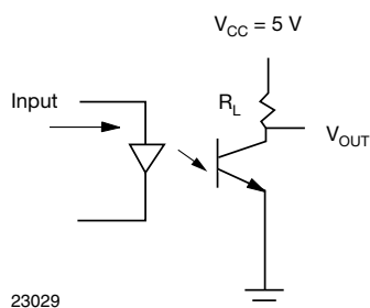
Fig. 2 - Test Circuit for Switching Characteristics
