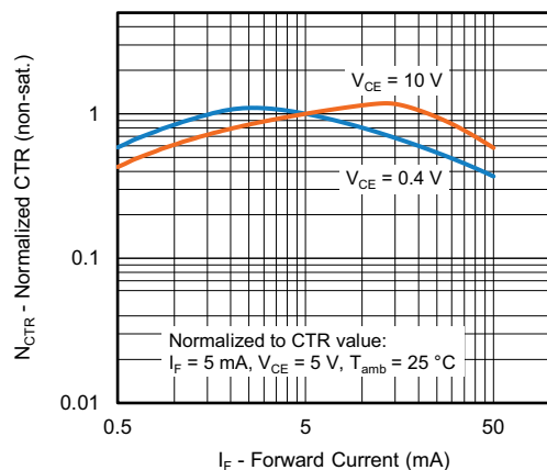
Fig. 6 - Normalized CRT vs. Forward Current (non-saturated)
