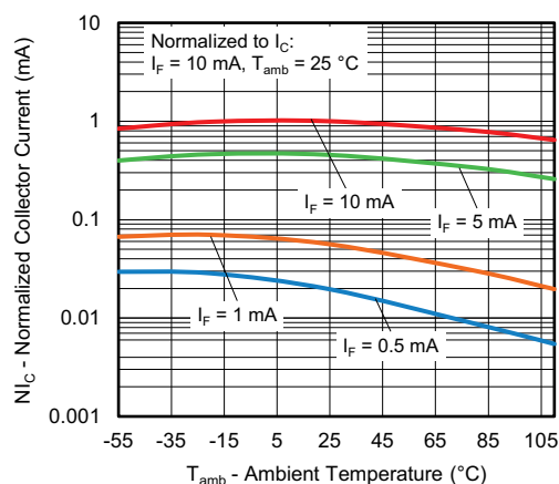
Fig. 7 - Normalized Collector Current vs. Ambient Temperature
