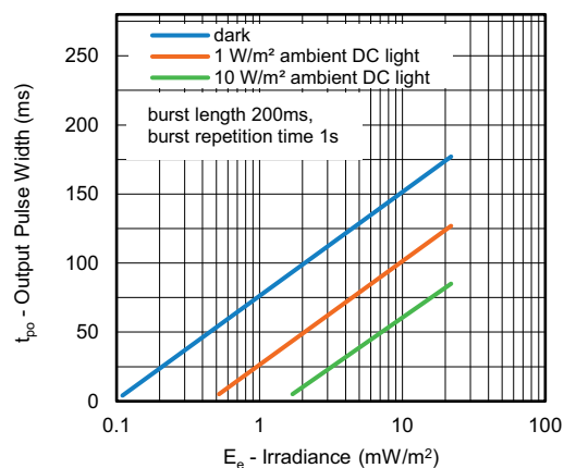
Fig. 6 - Output Pulse Width vs. Irradiance
