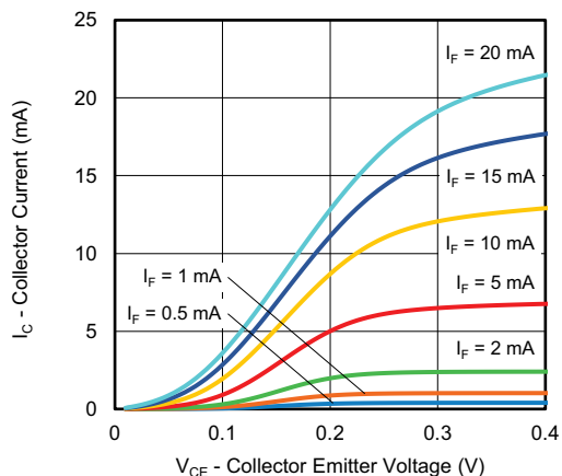
Fig. 9 - Collector Current vs. Collector Emitter Voltage (sat.)
