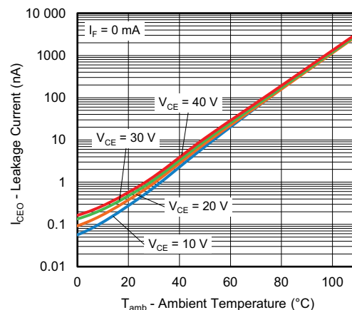
Fig. 12 - Leakage Current vs. Ambient Temperature
