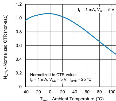
Fig. 10 - Normalized CTR (non-sat.) vs. Ambient Temperature
