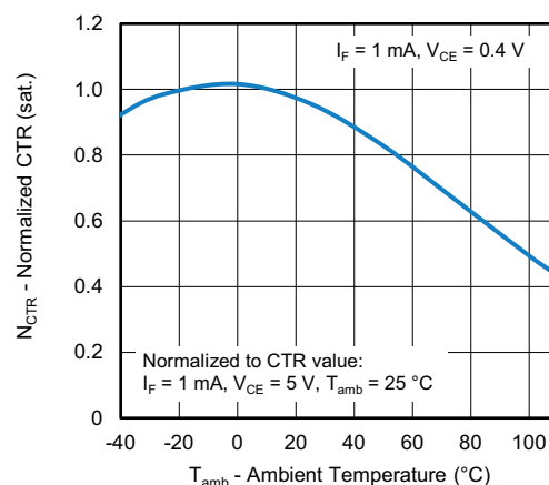
Fig. 11 - Normalized CTR (sat.) vs. Ambient Temperature
