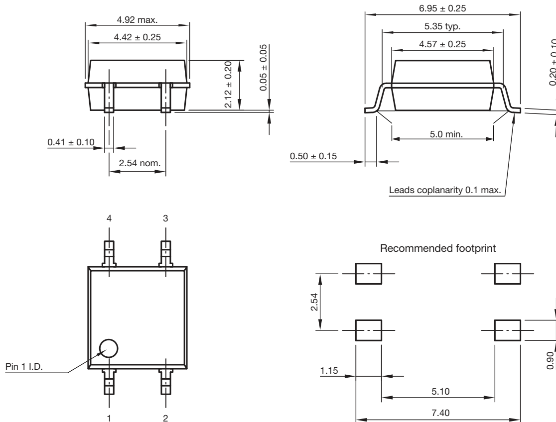
Fig. 18 - Package Drawing
