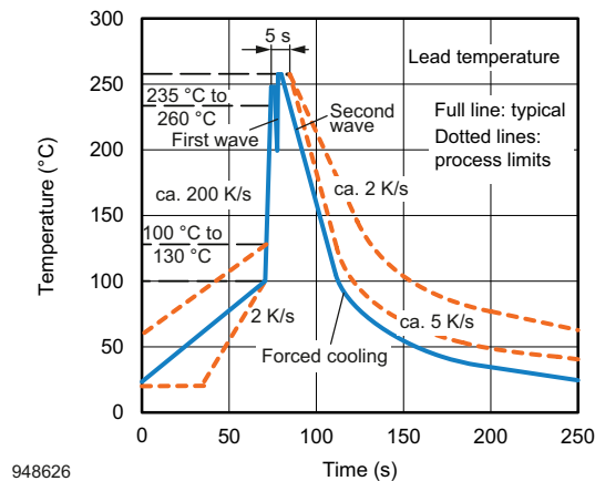
Fig. 9 - Wave Soldering Double Wave Profile According to J-STD-020 for DIP-8 Devices
