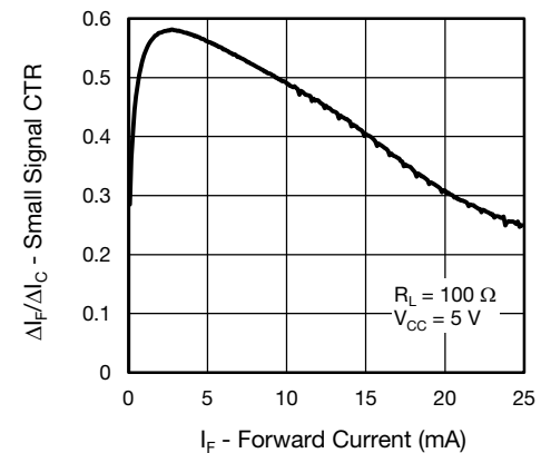
Fig. 9 - Small Signal Current Transfer Ratio vs. Forward Current
