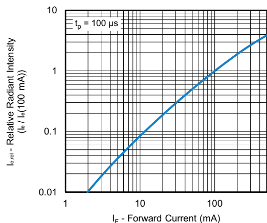
Fig. 4 - Relative Radiant Intensity vs. Forward Current
