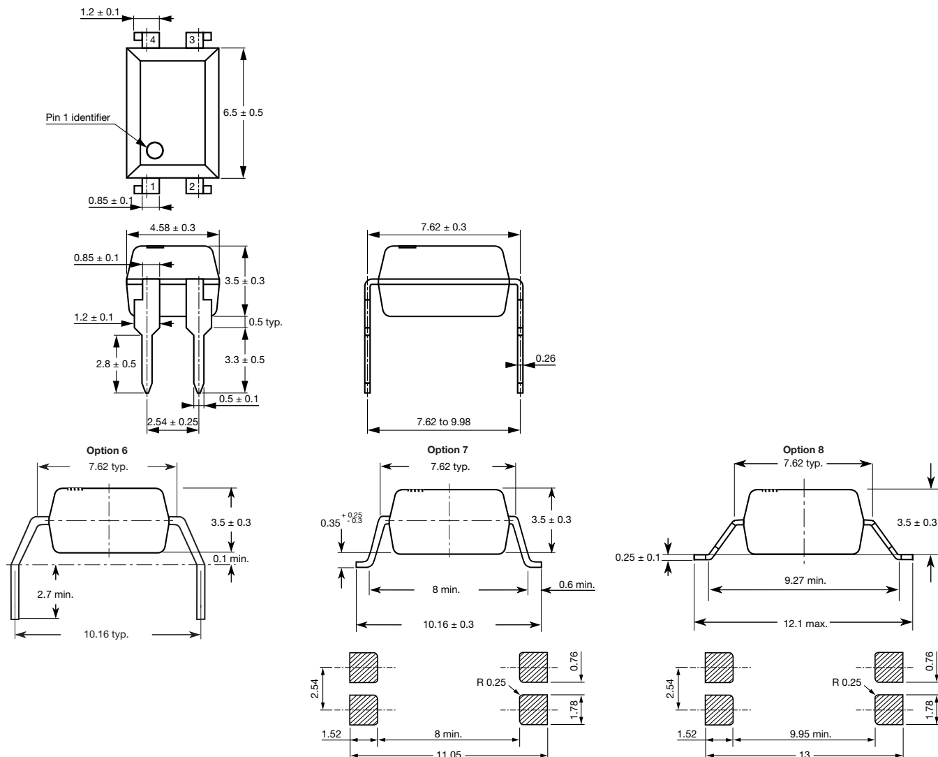
Fig. 17 - Package Drawings
