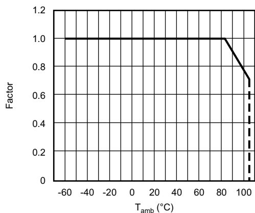
RMS voltage in function of temperature
