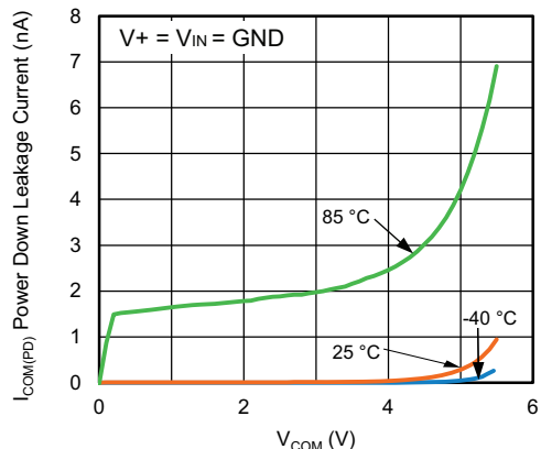
Power Down Leakage Current vs. V_{COM}
