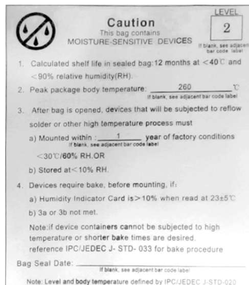
Example of JESD22-A112 level 2 label
