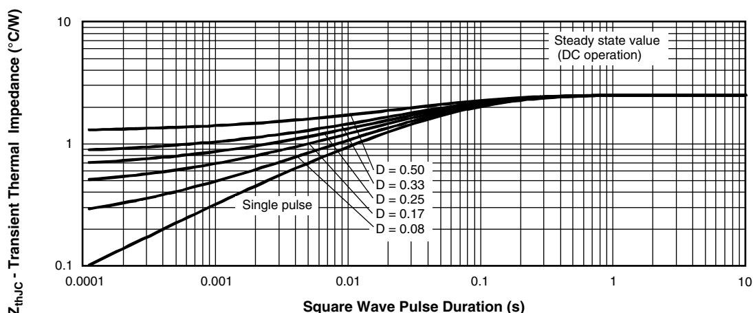
Fig. 8 - Thermal Impedance Z_{th,IC} Characteristics
