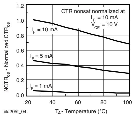
Fig. 8 - Current Transfer Ratio (normalized) vs. Ambient Temperature
