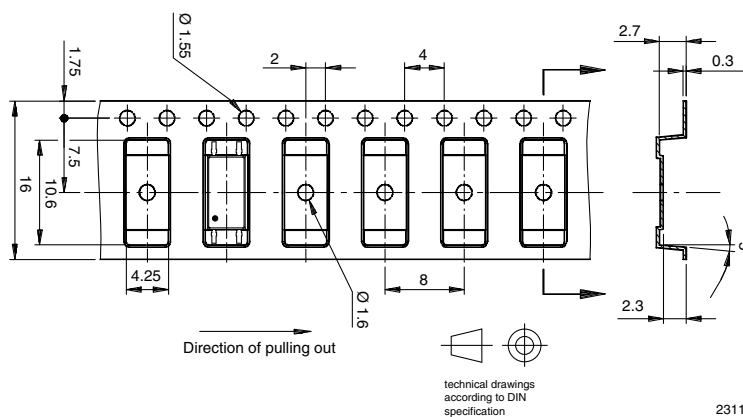
Fig. 21 - Tape and Reel Packing for VOL617A-xT3
