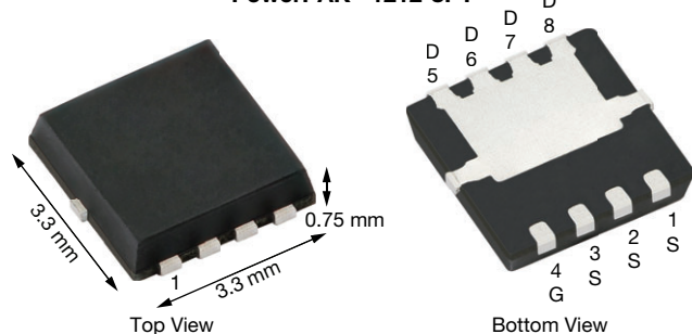
PowerPAK® 1212-8PT
