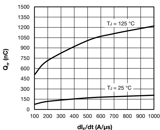
Fig. 16 - Typical Diode Reverse Recovery Charge vs. dl_F/dt I_F = 50 \text{ A} , V_{CC} = 200 \text{ V}
