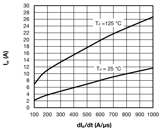
Fig. 15 - Typical Diode Reverse Recovery Current vs. dl_F/dt I_F = 50 \text{ A} , V_{CC} = 200 \text{ V}
