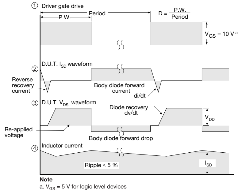
Fig. 14 - For N-Channel
