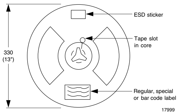
Fig. 15 - Tape and Reel Shipping Medium
