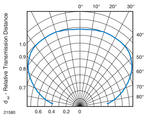
Fig. 12 - Vertical Directivity
