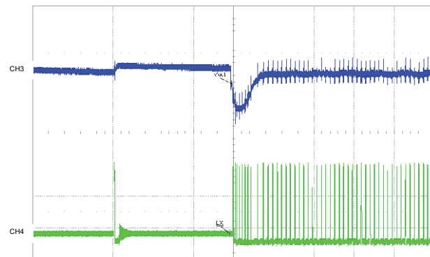
Fig. 9 - Load Step Undershoot Response, I_{OUT} = 0\text{ A} to 4 A, CH3 (BLU) = V_{OUT} (100 mV/div), CH4 (GRN) = LX (5 V/div), Time = 10 \mu\text{s/div}
