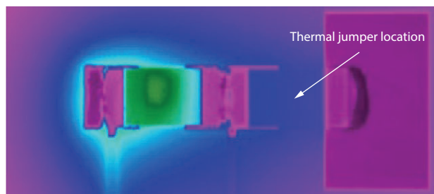
Ceramic Chip Resistor With Thermal Jumper (95.5 °C)
