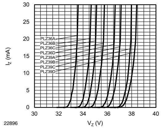
Fig. 12 - Breakdown Characteristics
