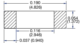
1505 Land Pattern
