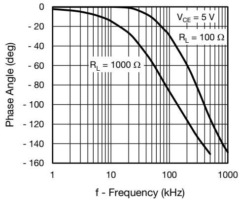
Fig. 14 - Frequency vs. Phase Angle
