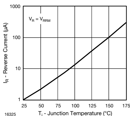
Fig. 4 - Reverse Current vs. Junction Temperature
